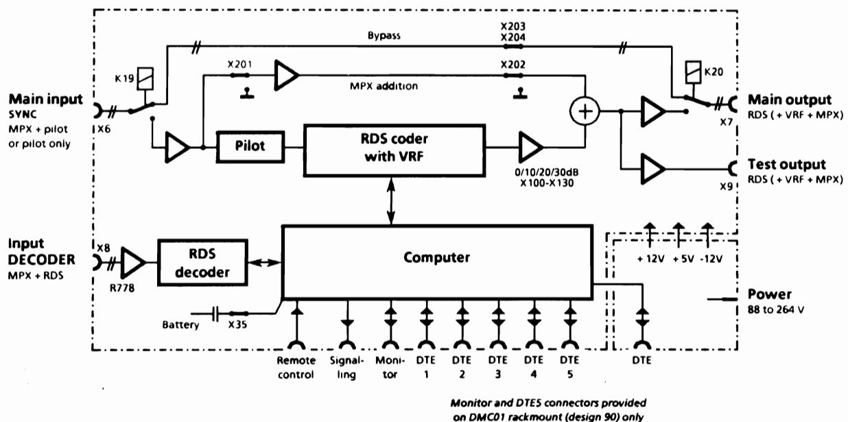
Fig. 2-1 Block diagram of DMC01 and DMC01C
